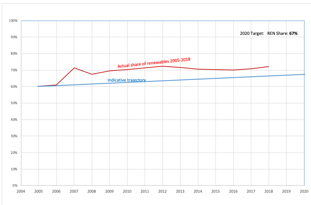
Figure 3 Actual share of renewable energy and indicative trajectory
